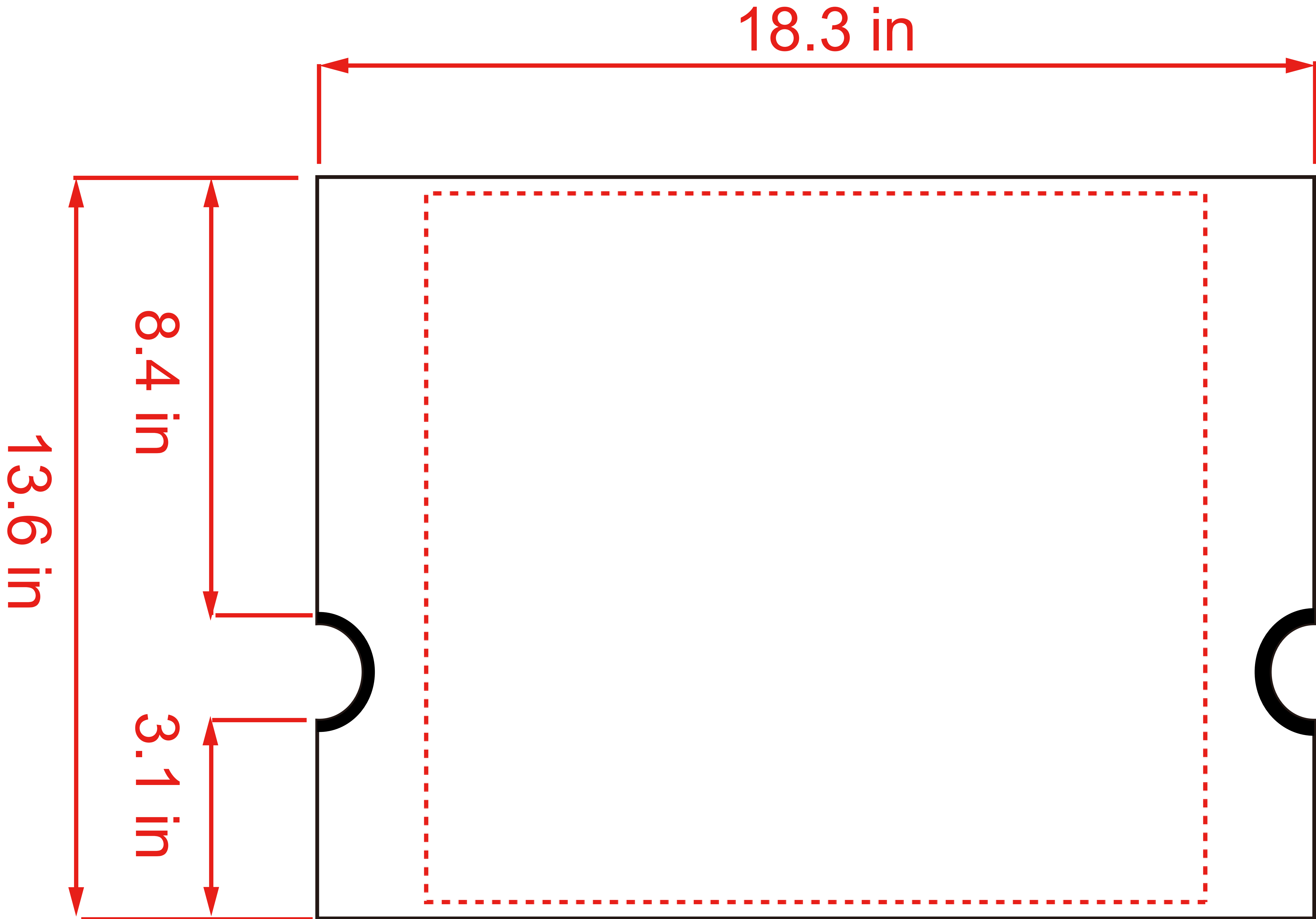
Backrest
