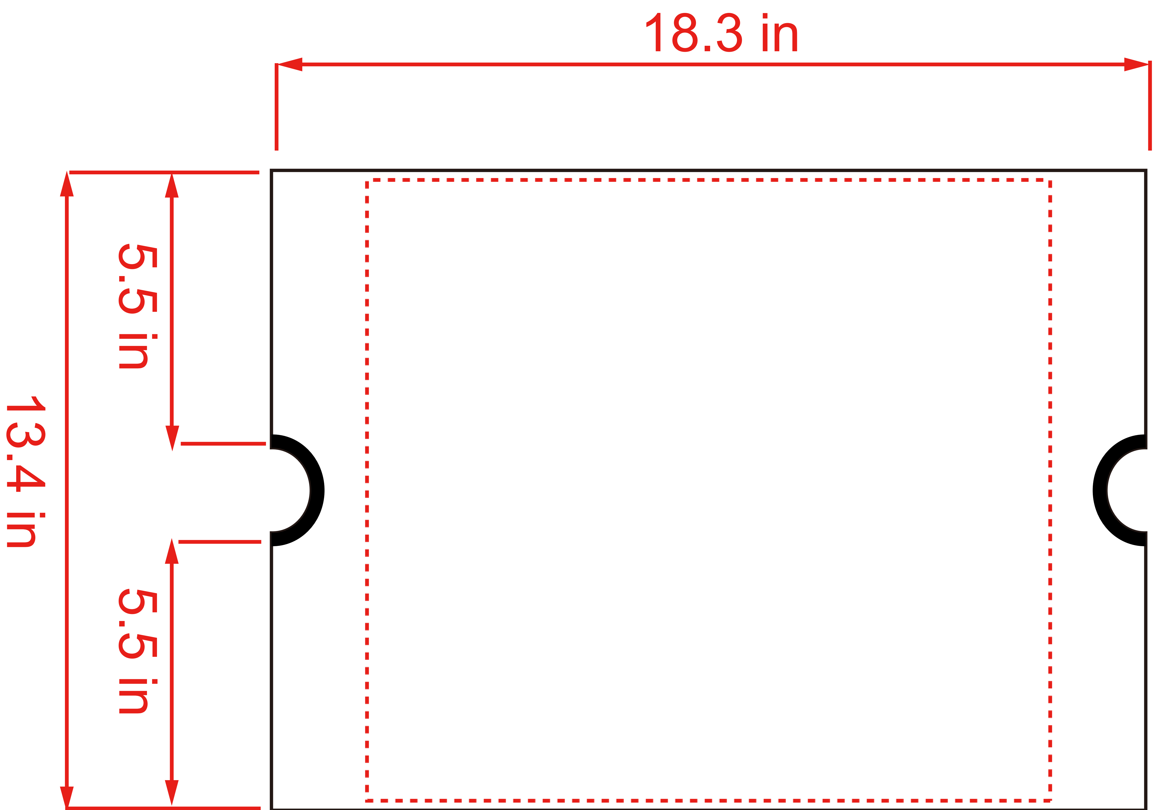
Seat Cushion
